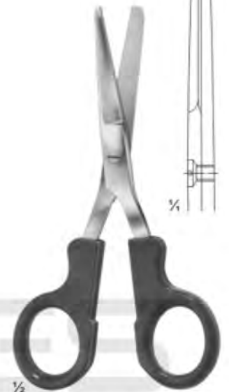
03-238 LISTER Nurse's scissors Size: 145 mm
